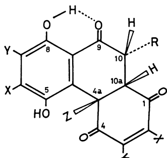
8 (Z=COCH 2 R) 4α-Acyl-10β-alkyl-5,8-dihydroxy-4α,10α-dihydro-1,4,9(10H)-phenanthrenetrione.
